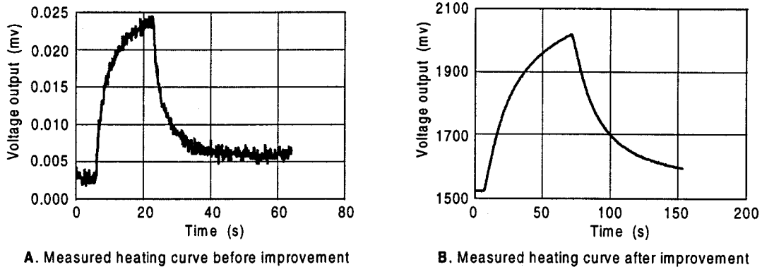
Figure 3 The heating curves measured before and after improvement.
