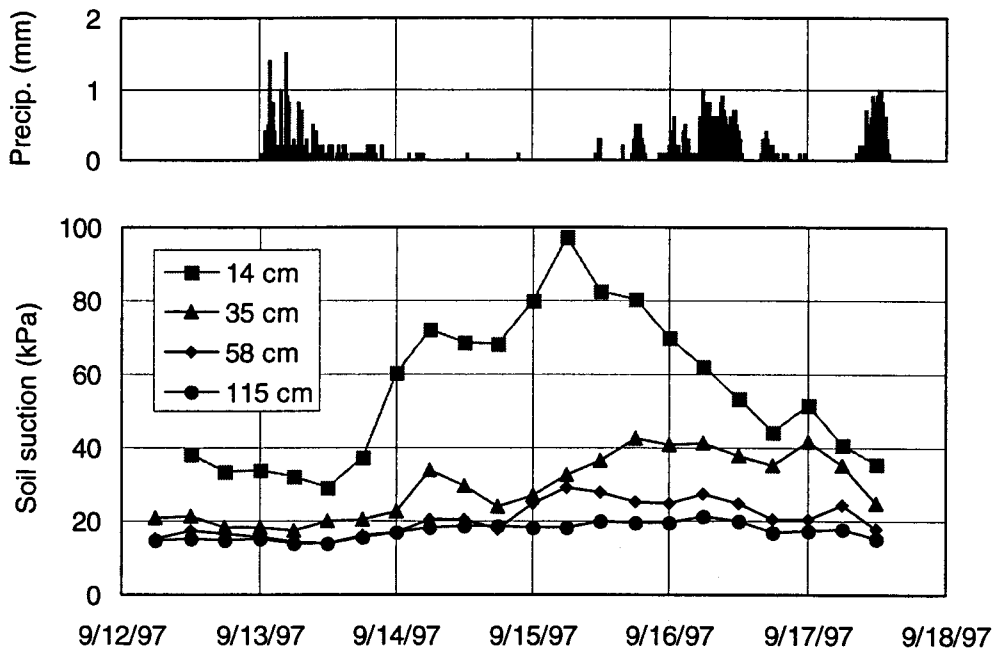
Figure 10 Soil suction measured in a test cover site
