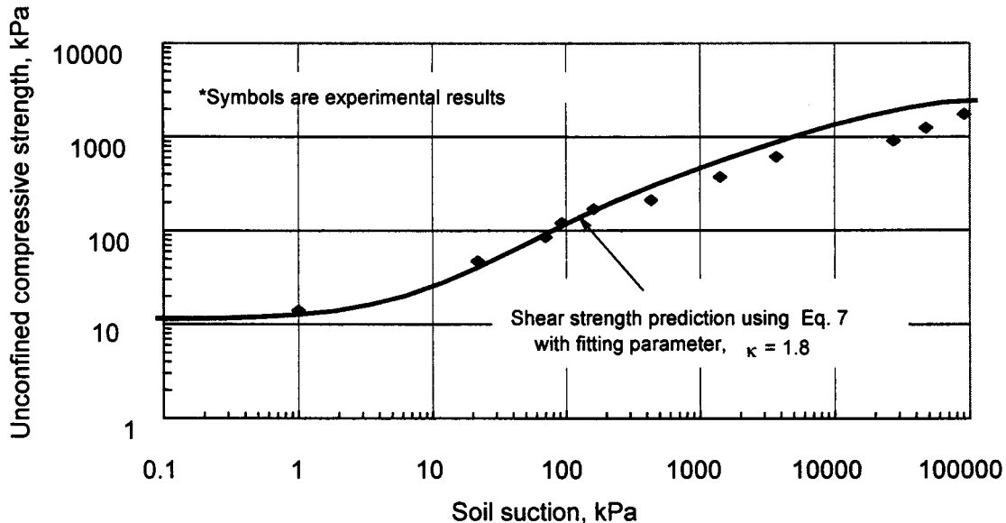
FIGURE 10. Comparison of between the measured and predicted unconfined compression strength test results.
