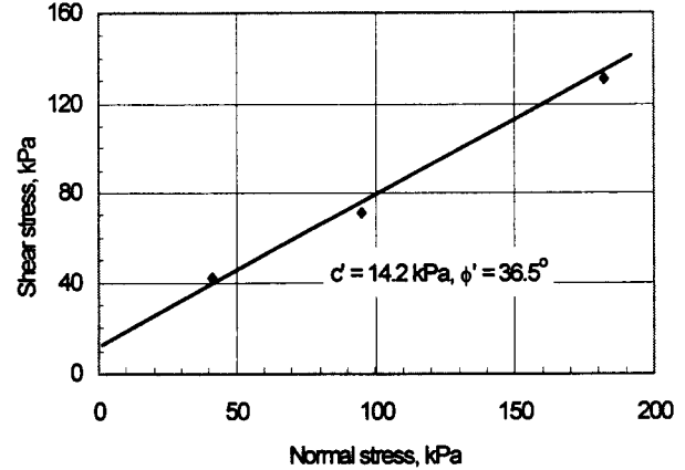
FIGURE 9. Direct shear test results to determine the saturated shear strength parameters of the Botkin silt
