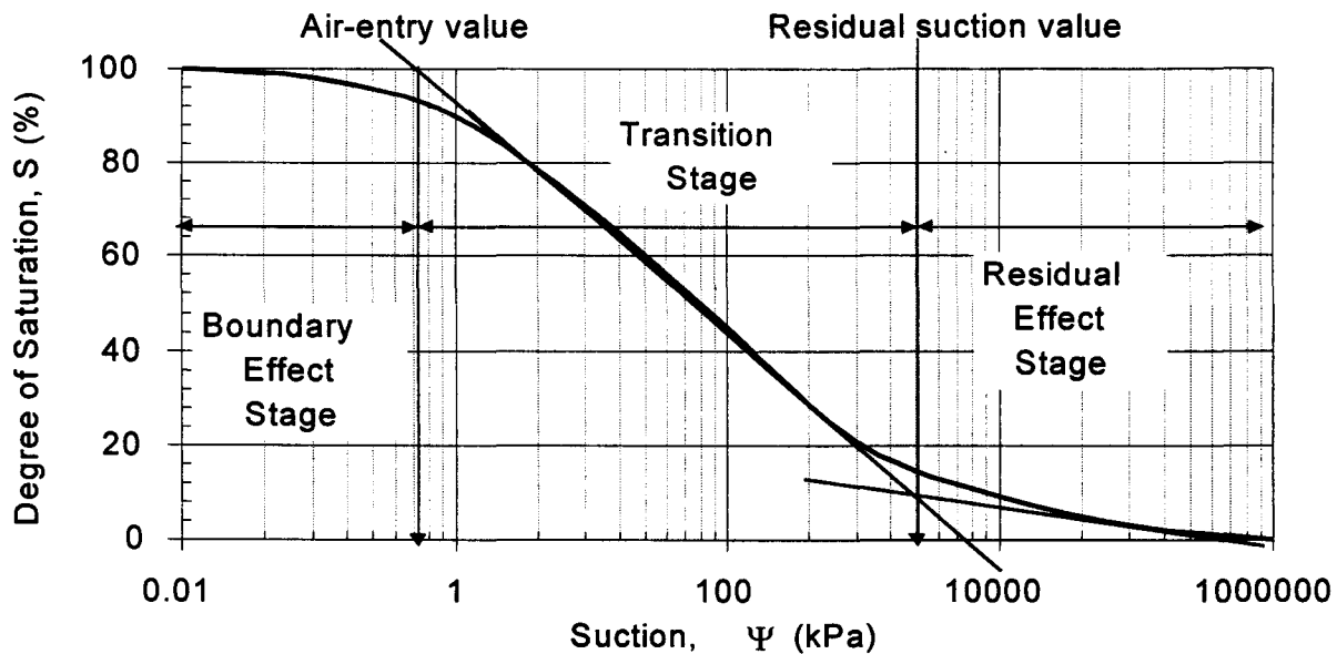
FIGURE 1. Typical soil-water characteristic curve showing various stages.
