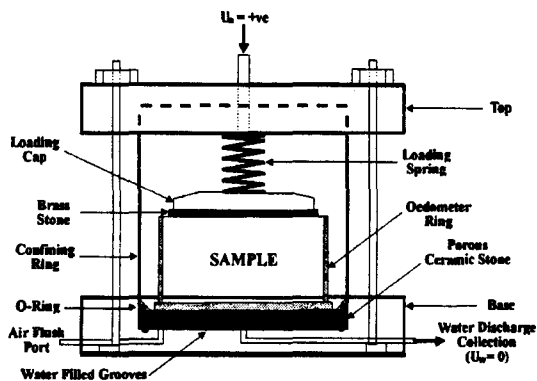
FIGURE 6. A modified pressure plate apparatus (i.e., Tempe cell) designed at the University of Saskatchewan for measuring the soil-water characteristic curve for a suction range between 0 to 500 kPa.
