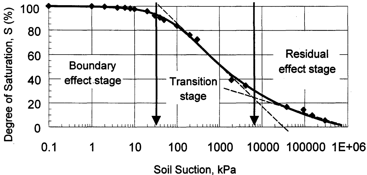
FIGURE 8. The entire soil-water characteristic curve for the tested Botkin silt.
