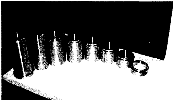
FIGURE 4. Specially designed molds for preparing specimens for unconfined compression testing.
