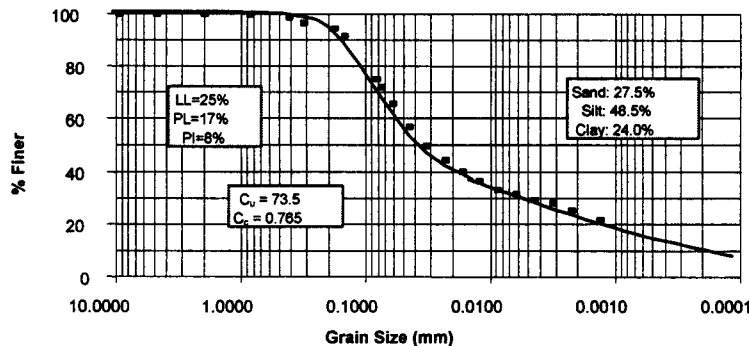
FIGURE 3. Grain size analysis for Botkin silt.
