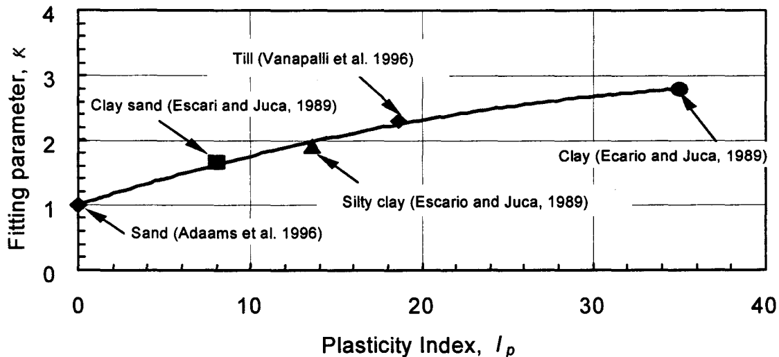
FIGURE 2. The relationship between the fitting parameter, \kappa , and the plasticity index, I_p . (from Vanapalli and Fredlund, 2000).
