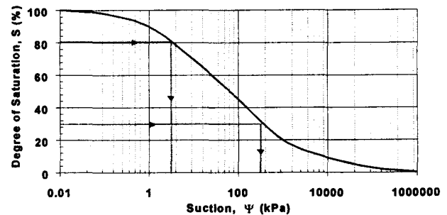
FIGURE 5. Indirect procedure for estimating the soil suction in the specimens knowing the degree of saturation.
