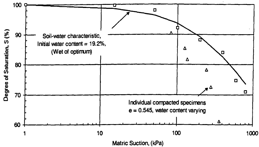
Figure 4. Comparison of soil-water characteristic curve for specimens compacted at wet of optimum initial water content and compacted at the same initial void ratio
