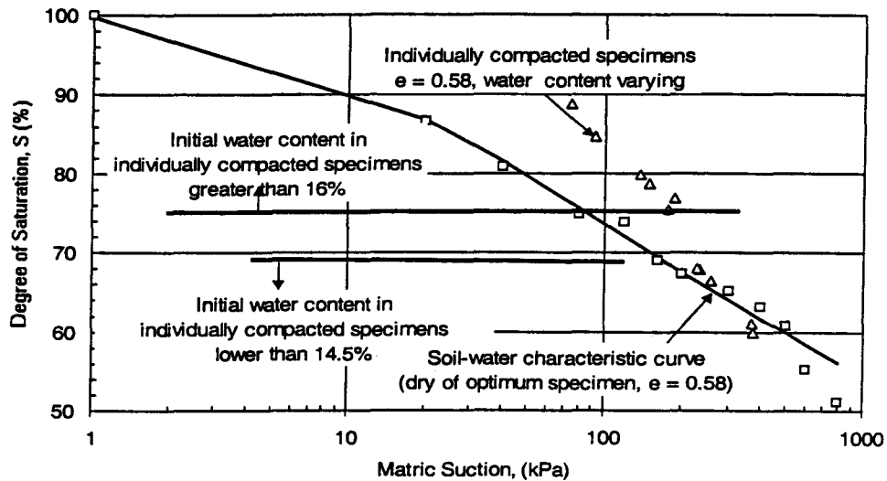
Figure 2. Comparison of soil-water characteristic curve for specimen compacted at dry of optimum water content and those compacted at the same initial void ratio
