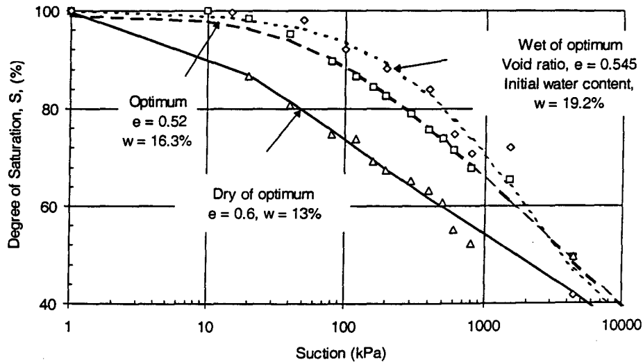
Figure 1. Soil-water characteristic curves for specimens compacted at three different initial water contents
