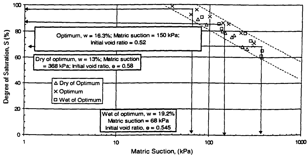
Figure 5. Degree of saturation versus matric suction values for compacted specimens
