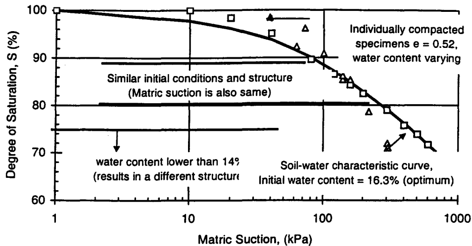
Figure 3. Comparison of soil-water characteristic curve for specimens compacted at optimum water content and those compacted at the same initial void ratio
