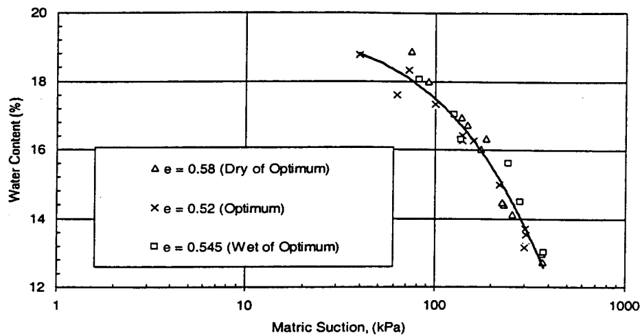
Figure 6. Gravimetric water content versus matric suction for compacted specimens
