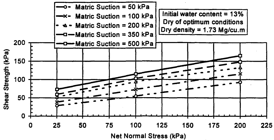
Figure 6. Variation of shear strength with net normal stress under different matric suctions for specimens with initial water contents dry of optimum.
