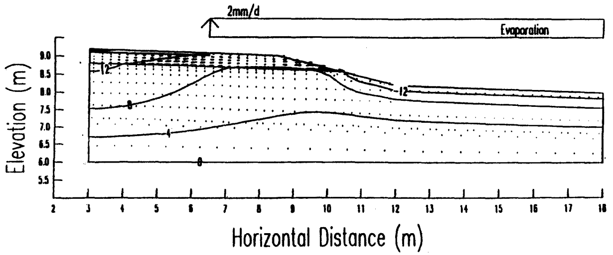
Figure 10a. Transient evaporation at time lapse of 1 day.
