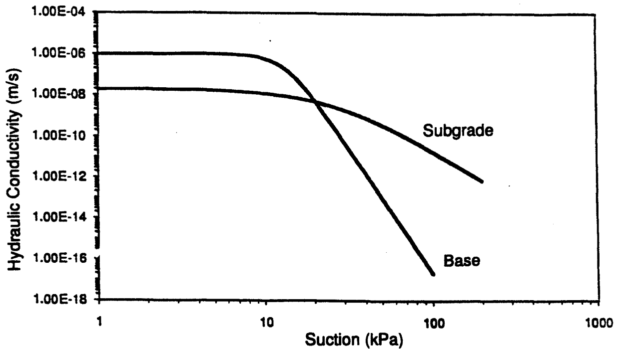
Figure 3. Hydraulic conductivity versus suction relationship.
