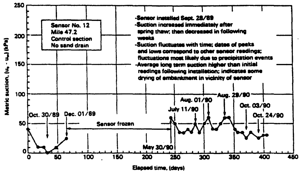
Figure 18. Matric suction readings from sensor No. 12.
