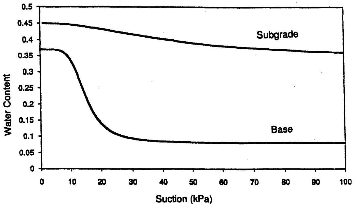
Figure 2. Volumetric water content versus suction relationships.
