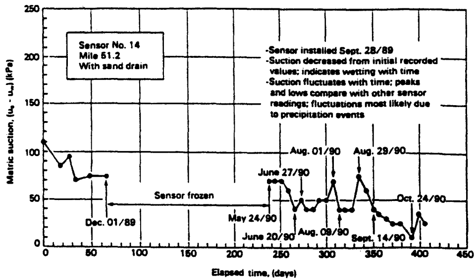
Figure 17. Matric suction readings from Sensor No. 14.
