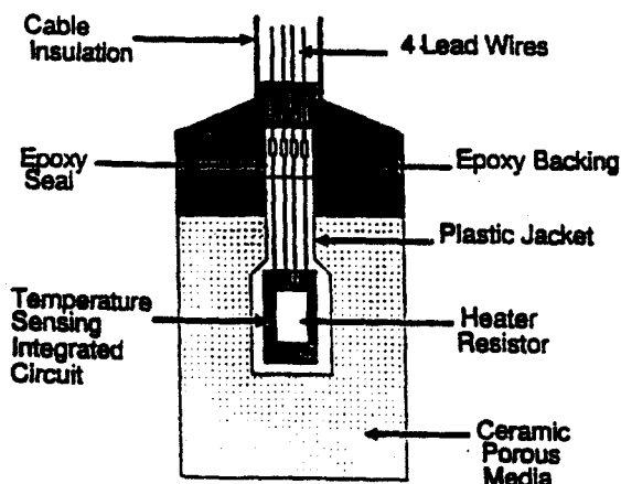
Figure 14. Schematic diagram of an integrated circuit type thermal conductivity matrix suction sensor.
