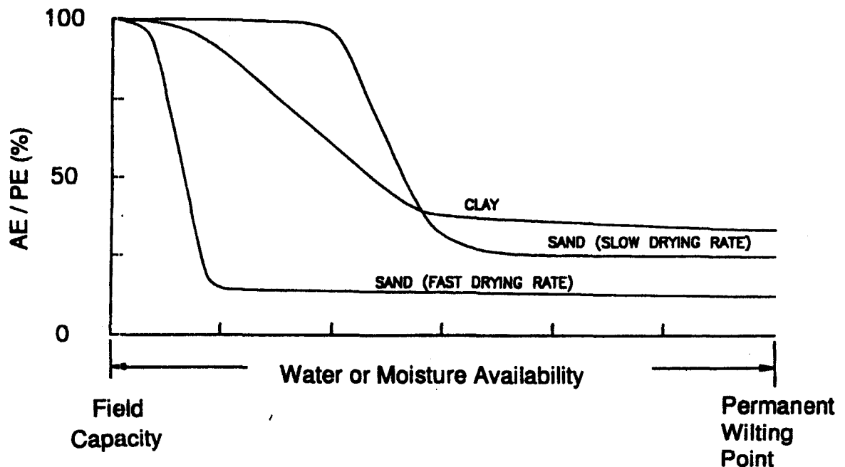
Figure 4. The ratio of the actual rate of evaporation and potential evaporation, AE/PE, versus water availability (after Holmes, 1961; and Gray, 1970).
