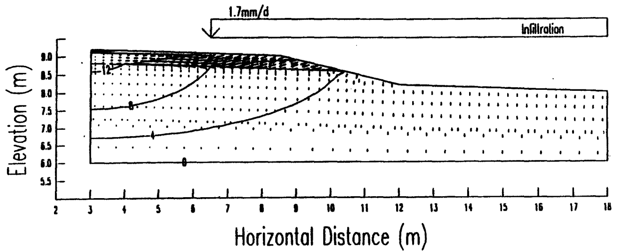
Figure 7. Steady state infiltration under a flux rate of 1.7 mm/day.
