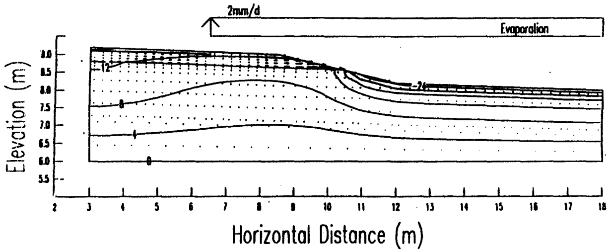
Figure 10b. Transient evaporation at time lapse of 4 days.
