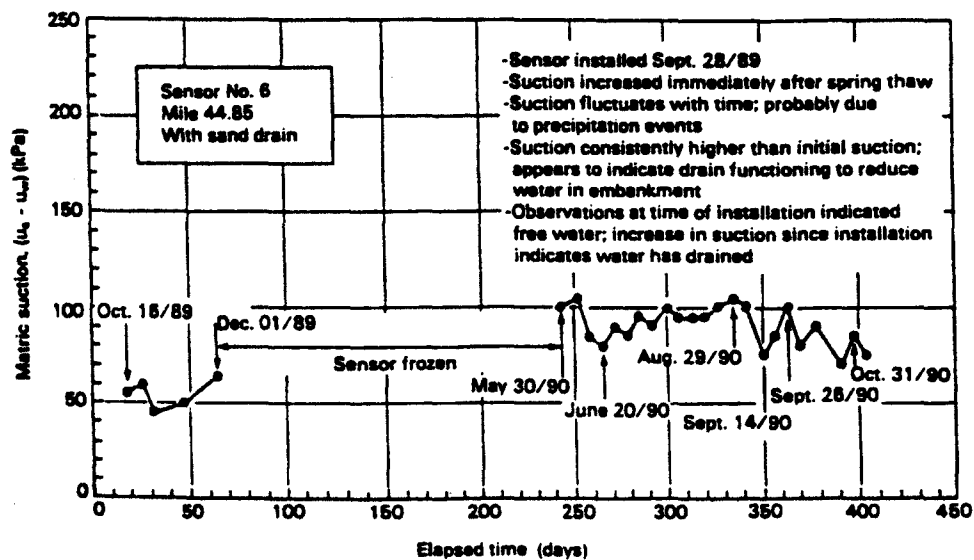
Figure 16. Matric suction readings from Sensor No. 6.
