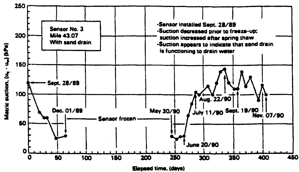
Figure 15. Matric suction readings from Sensor No. 3.
