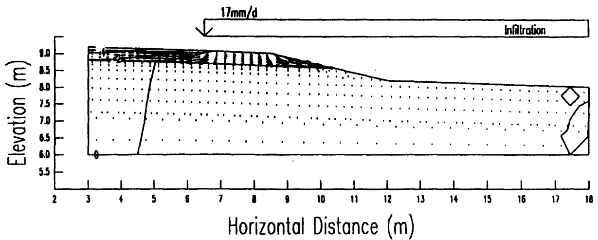
Figure 8. Steady state infiltration under a flux rate of 17 mm/day.
