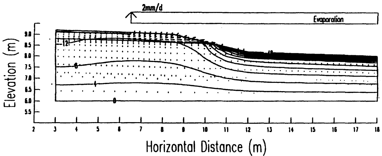
Figure 10c. Transient evaporation at time lapse of 10 days.
