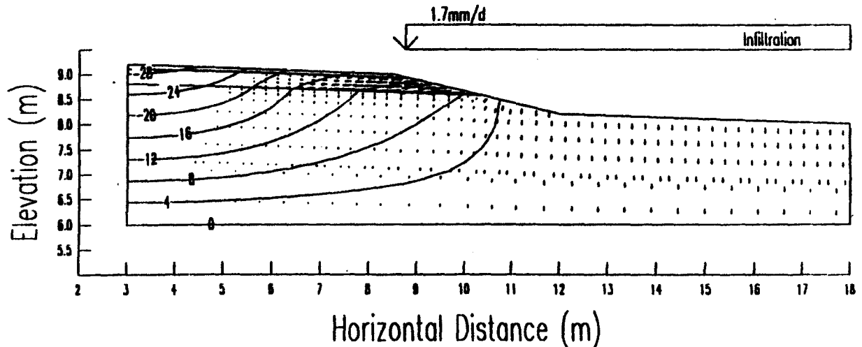
Figure 13. Steady state infiltration through roadway with paved asphalt shoulder.
