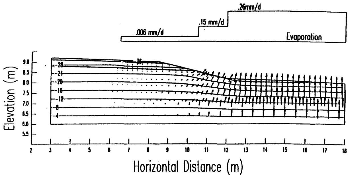
Figure 9. Steady state evaporation.
