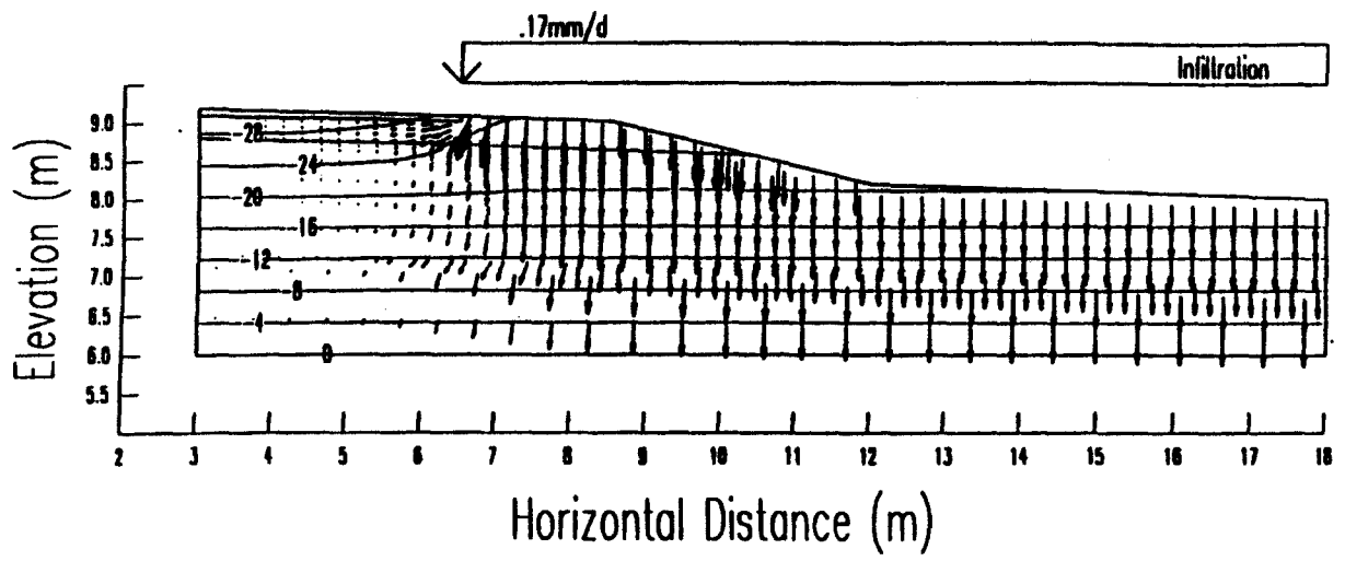
Figure 6. Steady state infiltration under a flux rate of 0.17 mm/day.
