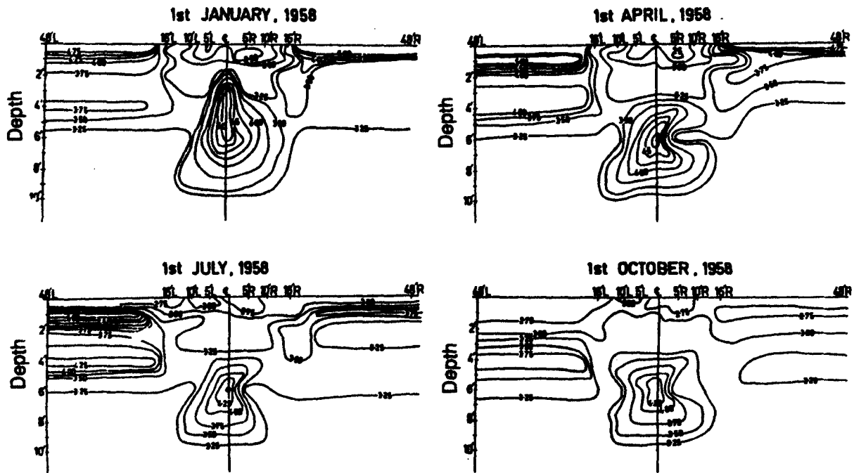
Figure 12. Seasonal suction distribution below a highway structure in Horsham, Australia (from Richards, 1965).
