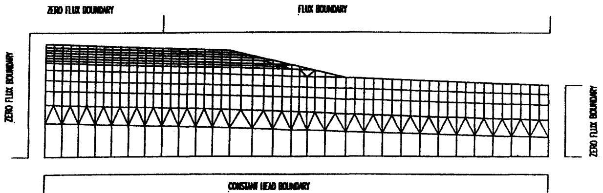
Figure 5. Finite element grid of highway cross-section.
