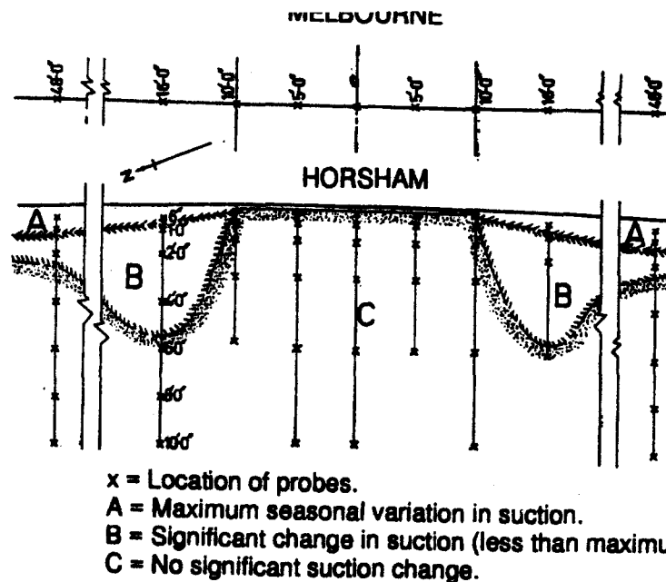
Figure 11. Typical suction distribution below a highway structure in Horsham, Australia (from Aitchison and Richards, 1965).
