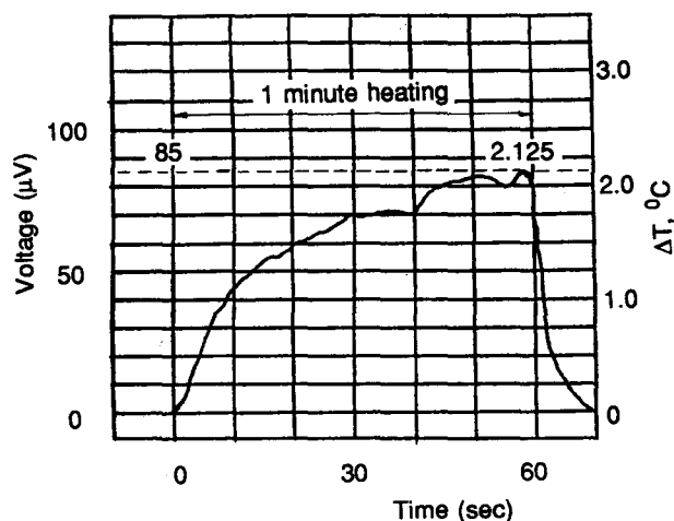
Fig. 9. Typical voltage output from an AGWA sensor which uses an IC type temperature sensing device.
