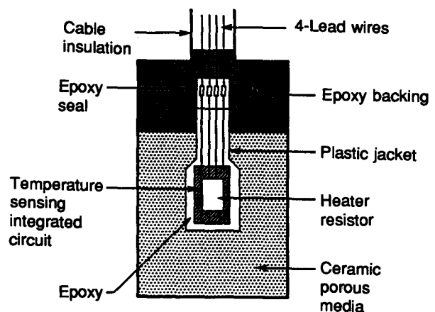
Fig. 1. A cross-sectional diagram of a thermal conductivity matric suction sensor showing its key components.
