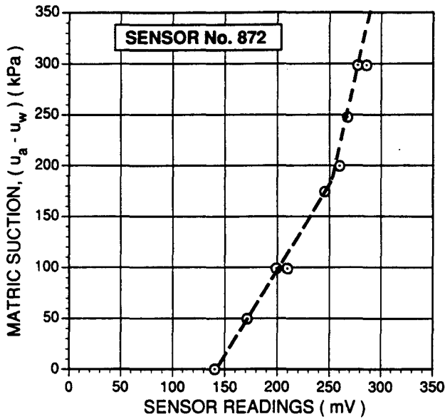
FIGURE 14 Typical thermal conductivity sensor calibration curve.
