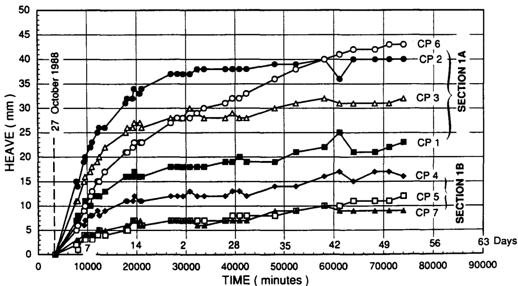
FIGURE 11 Heave measurements in Sections 1A and 1B.
