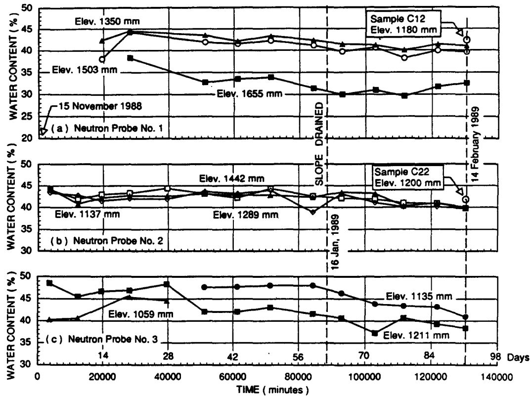
FIGURE 12 Neutron probe water content and gravimetric water content measurements in Section 1A.
