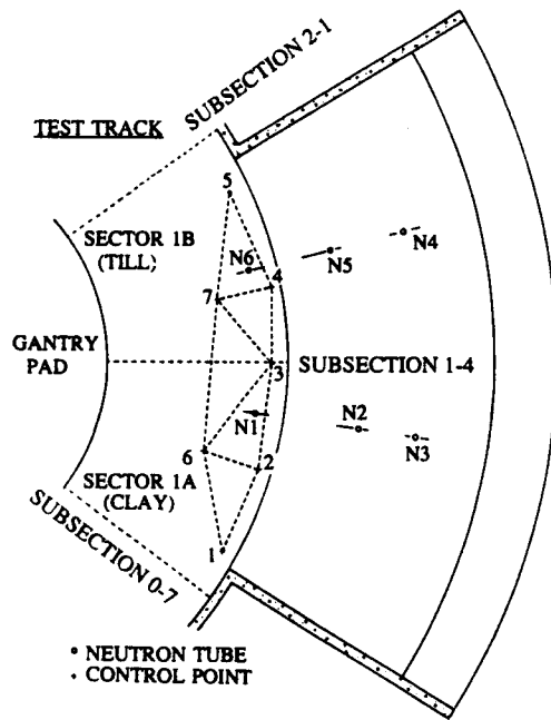
FIGURE 4 Location of neutron tubes and survey control points.
