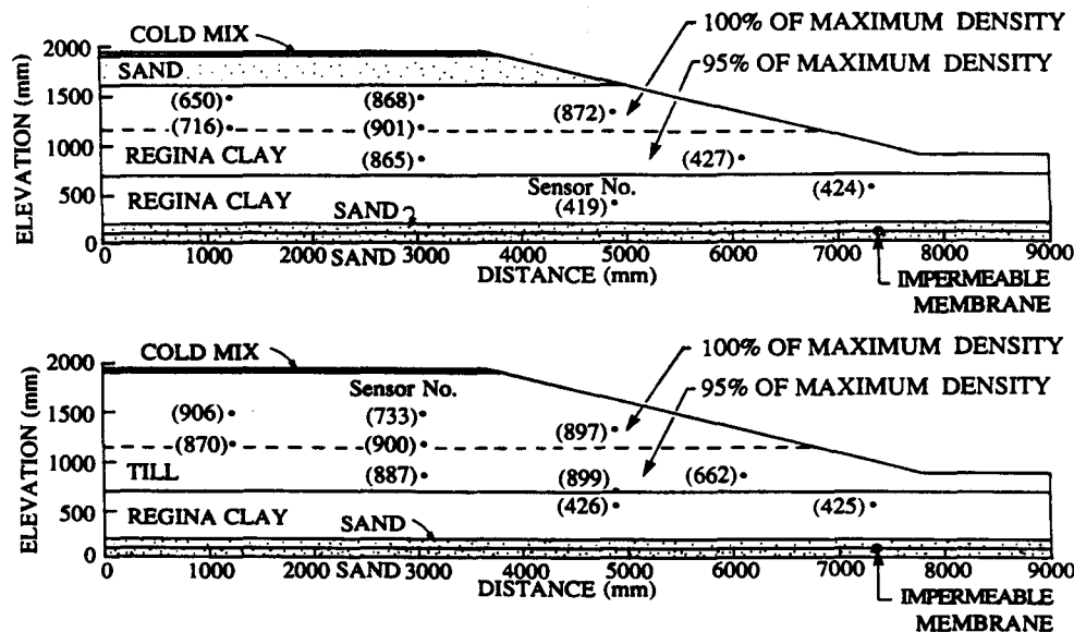
FIGURE 3 Location of thermal conductivity sensors in Sections 1A and 1B.
