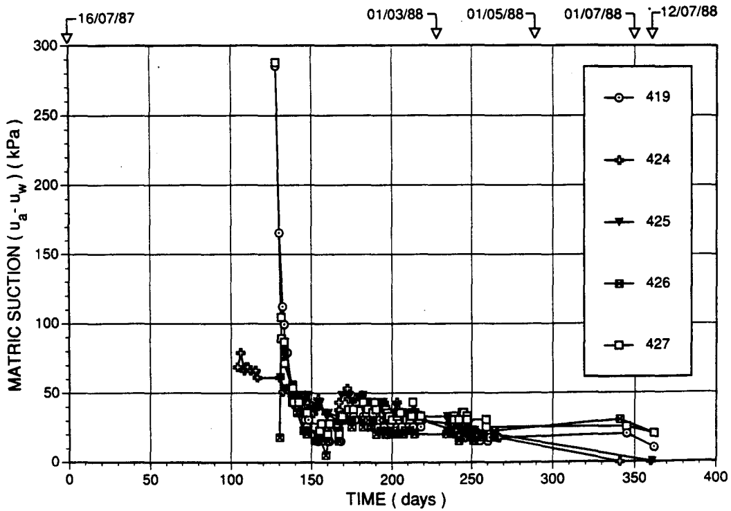
FIGURE 8 Long-term matric suction readings from thermal conductivity sensors installed in pretwetted holes.
