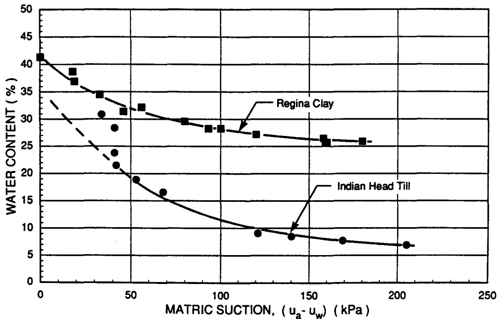
FIGURE 6 Water content-versus-matric suction relationships of slurried samples of Regina clay and Indian Head till.
