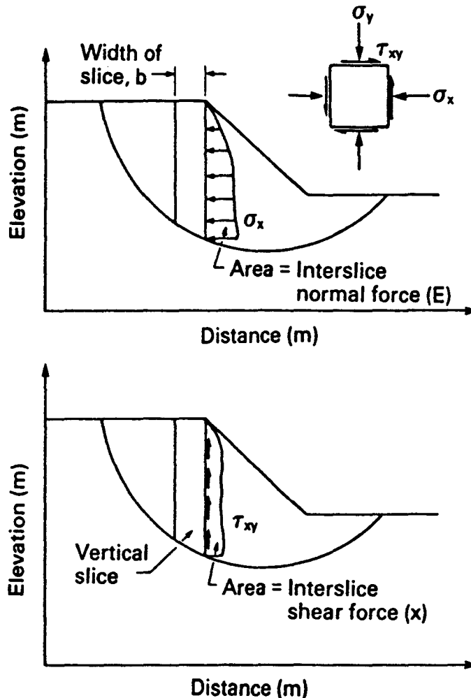
Fig. 4 The normal and shear forces acting on the right side of a slice
