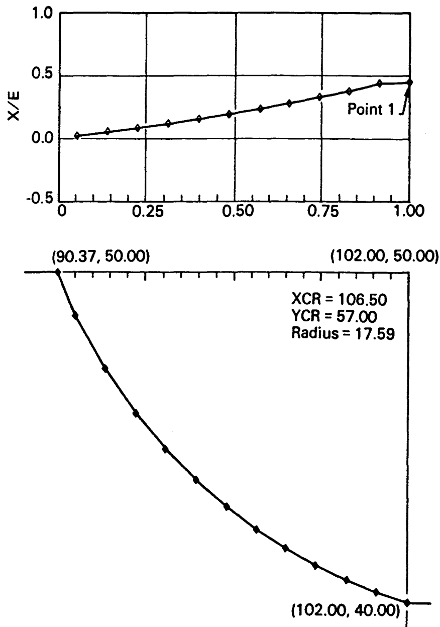
Fig. 7 The interslice side force ratio distribution for the active case ( \phi = 30^\circ ; \delta = 15^\circ )
