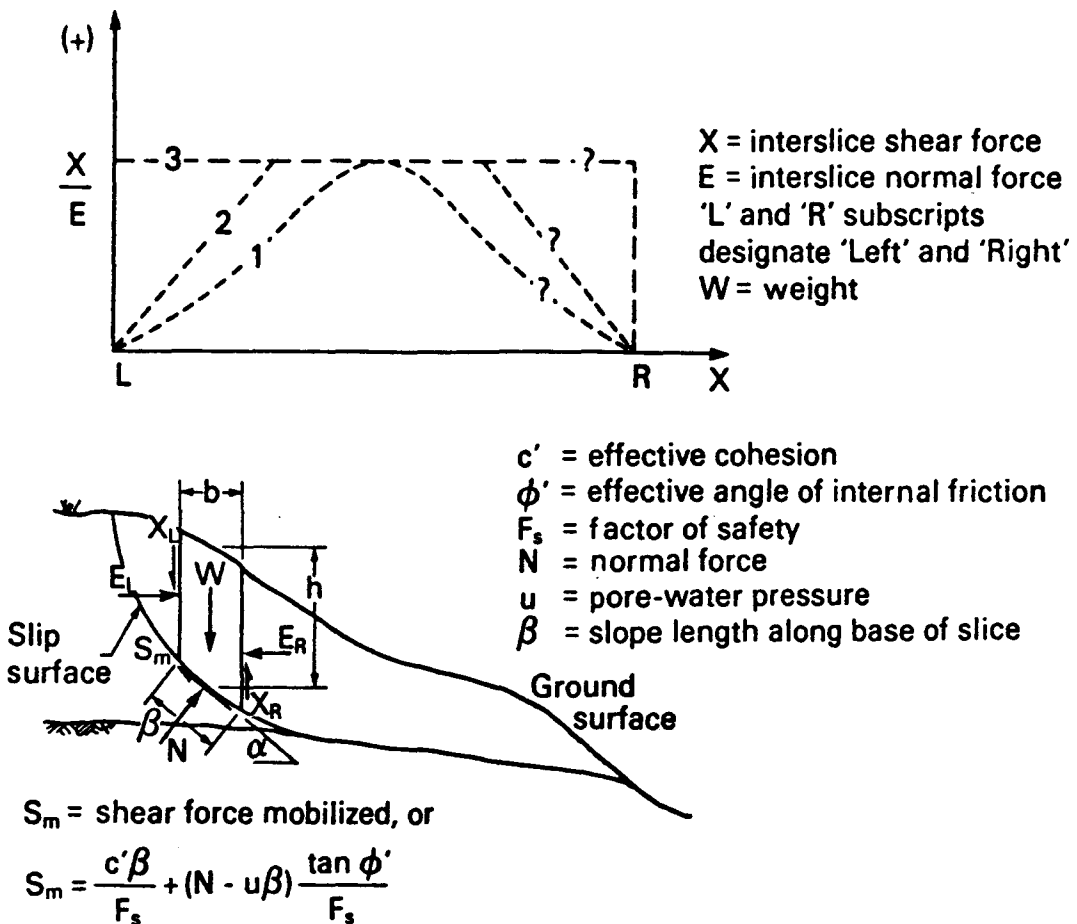
Fig. 1 Assumed interslice force functions for slope stability
