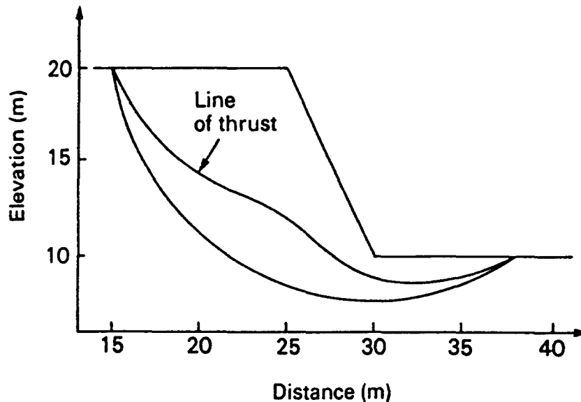
(b) Resulting line of thrust
