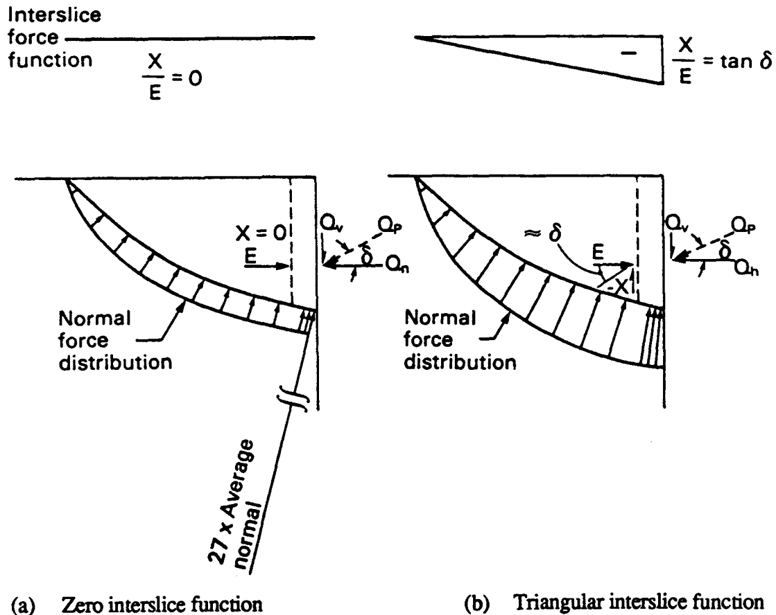
Fig. 3 Effect of the interslice force function on the normal force distribution (passive case)
