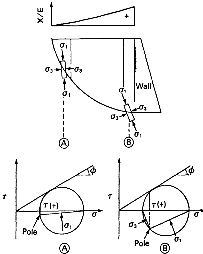
Fig. 8 The interslice force function and the orientations of the principal planes for the active case
