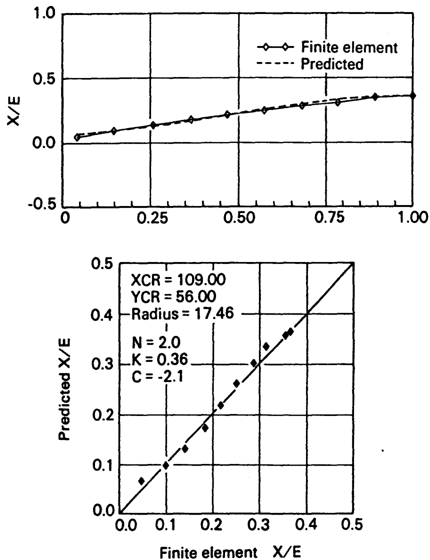
Fig. 11 X/E computed by the generalized function (predicted) versus X/E computed by the finite element method in the active case
