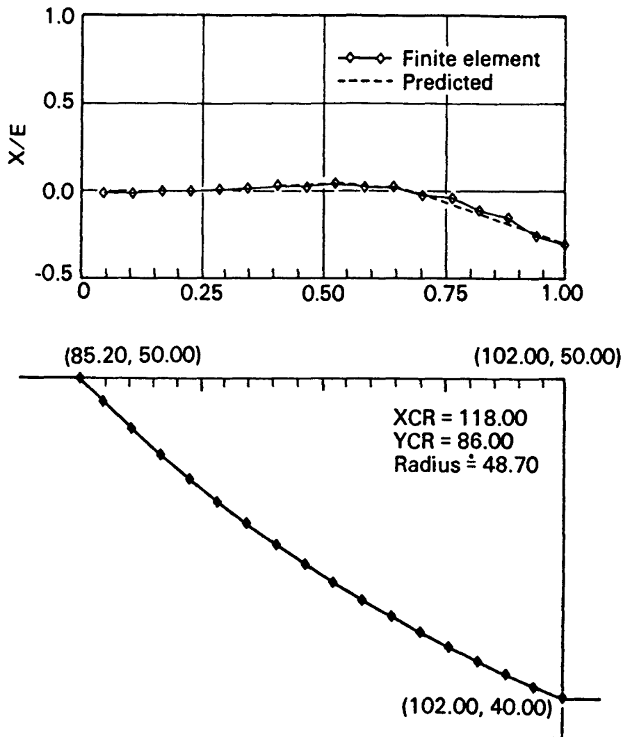
Fig. 12 X/E computed by the straight line approximation method (predicted) versus X/E computed by the finite element method in the passive case
