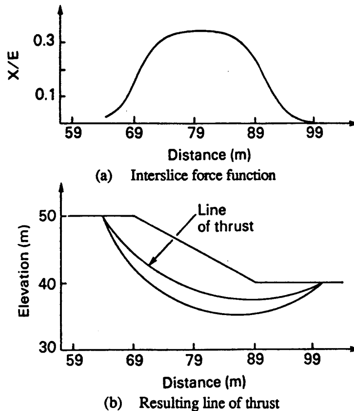
Fig. 5 Interslice force function for a deep-seated slip surface in a 2:1 slope
