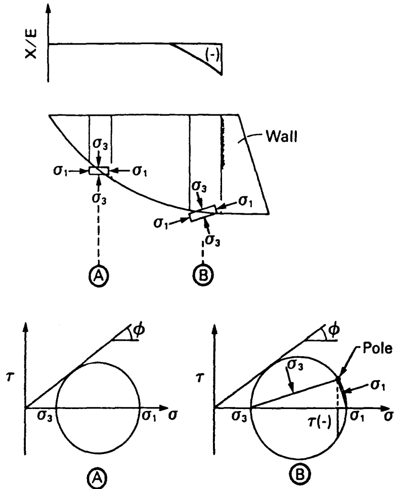
Fig. 10 The interslice force function and the orientations of the principal planes for the passive case.
