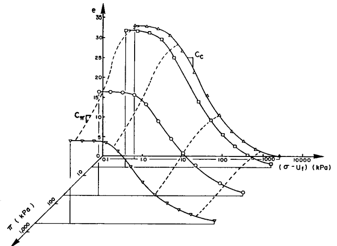
Figure 2. Three dimensional constitutive surface for Na-montmorillonite as drawn from the data of Mesri and Olson (1971).
