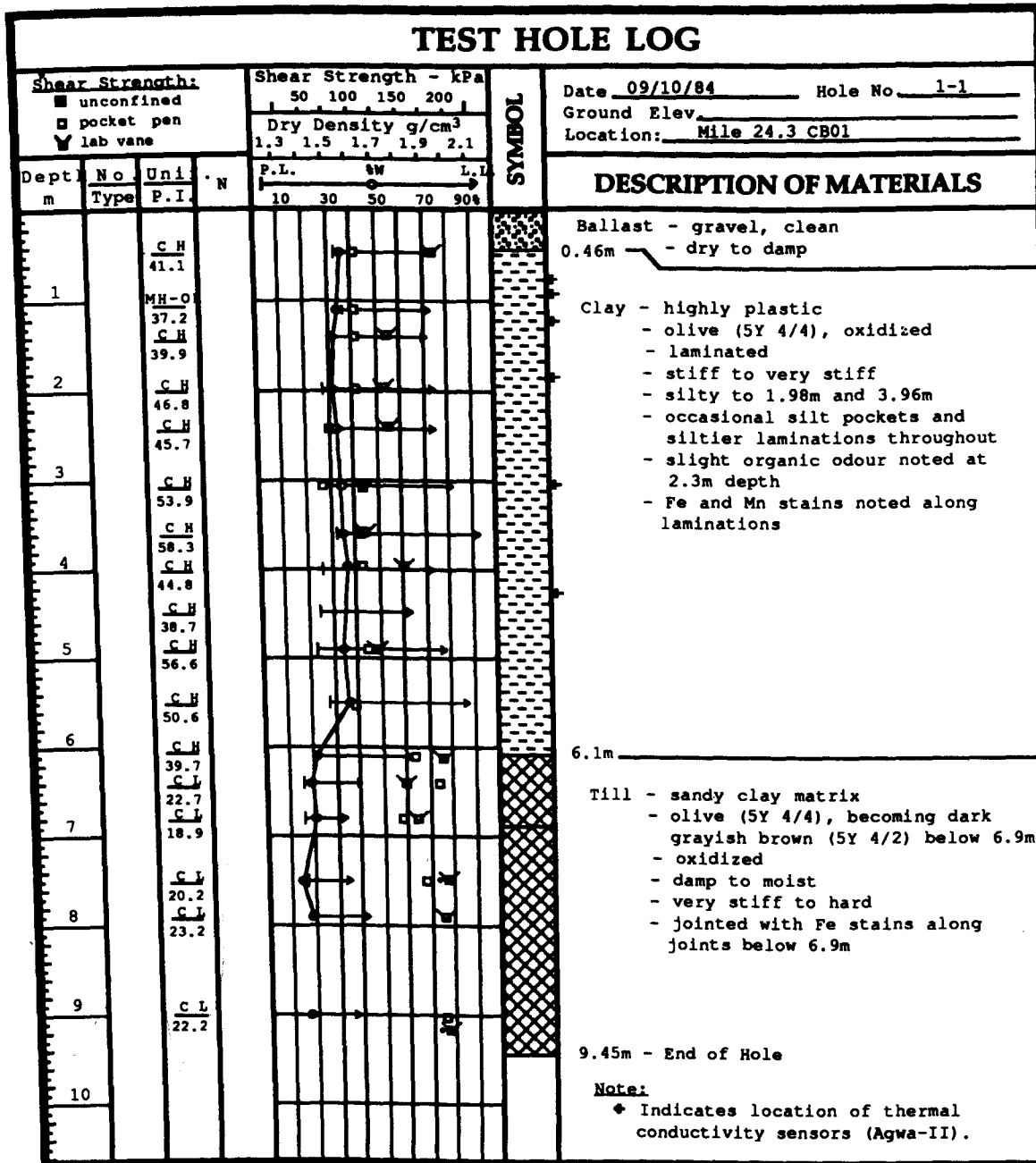
FIGURE 5 Test hole information from Site No. 1, Belle Plaine.
