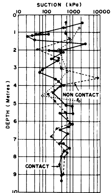
FIGURE 8 Suction versus depth for test hole No. 1 using the McQueen and Miller filter paper method.
