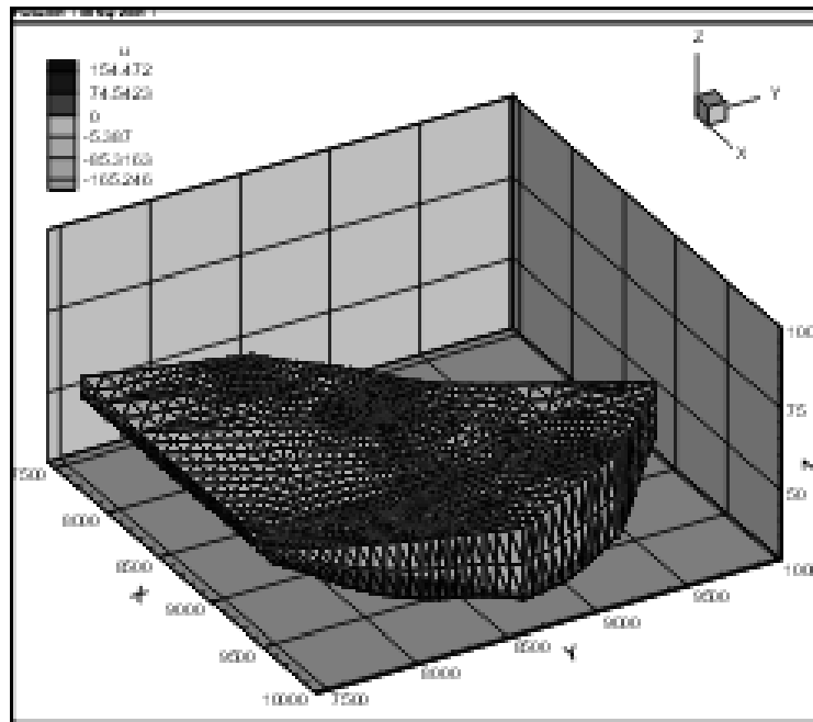
Figure 3. Representation of SVFluxTM finite element results of pressure head at steady state (pressure, u (kPa); dimensions (m)).
