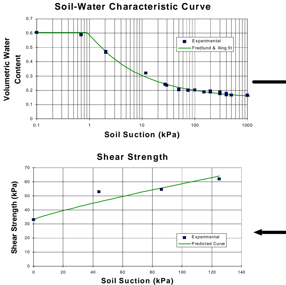
Figure 3 Plot of predicted shear strength envelope for a Sandy Clay Loam
