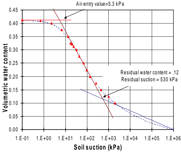
Figure 5 Results of the construction technique for a Silt Loam (from van Dam et al. 1992) (SoilVision soil #133)
