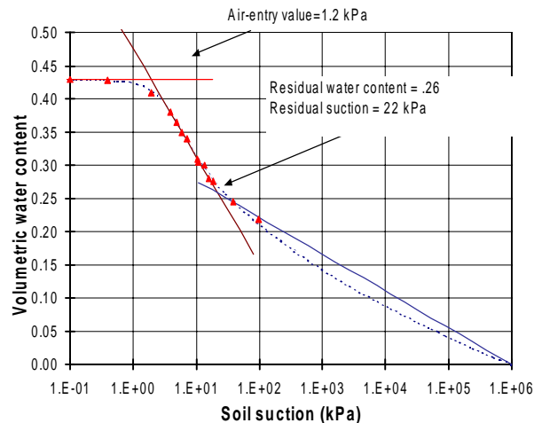
Figure 4 Results of the construction technique for a Loam (from Sisson and van Genuchten, 1991) (SoilVision soil #131)
