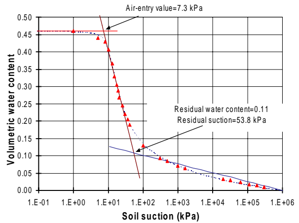
Figure 3 Results of the construction technique for a Loam (from Jackson et al. 1965) (SoilVision soil #91)
