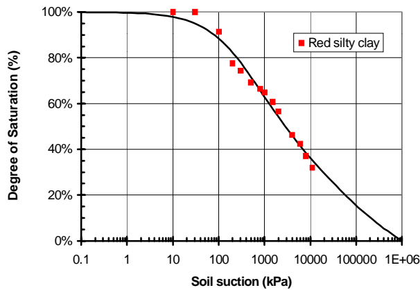
Figure 6 Soil-water characteristic curves for Madrid clayey sand and Guadalix Red silty clay (modified after Escario and Juca 1989).
