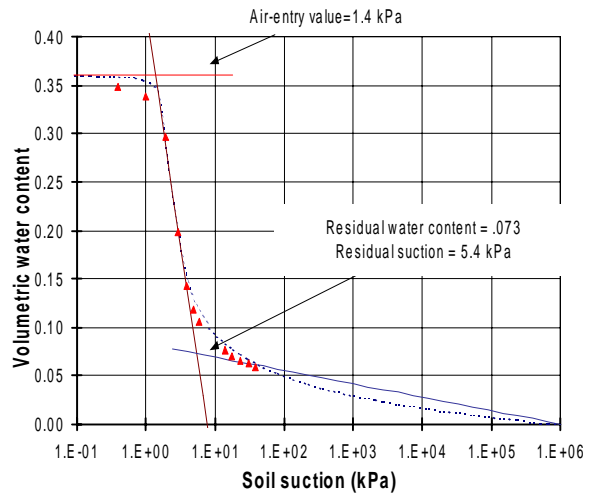
Figure 2 Construction procedure to estimate the residual state and the air-entry value of a Sand. (from Dane et al. 1983) (SoilVision soil #10723)
