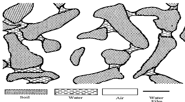
Figure 1 The probable soil-water-air interphase relationship at residual state condition (after Fairbridge and Finkl 1979)
