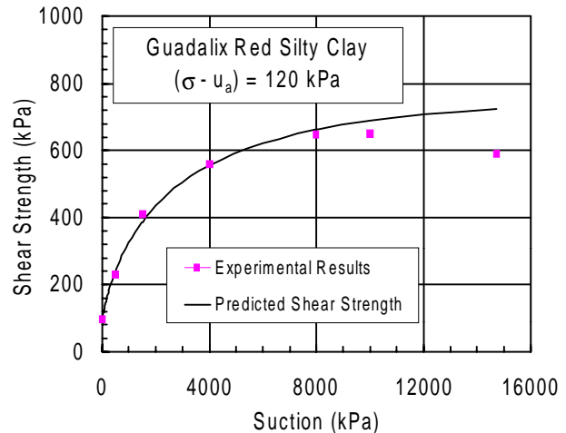
Figure 7. Measured and predicted shear strength values for Guadalix Red silty Clay
