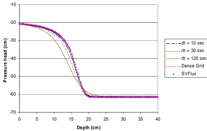
Figure 1 Comparison between SVFLUX and Haverkamp (1977) as presented by Celia (1990)
