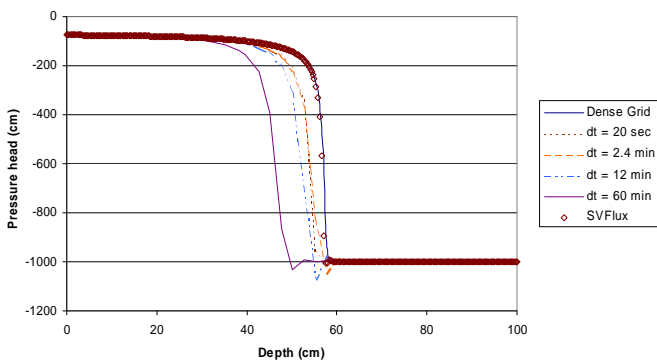
Figure 2 Comparison between SVFLUX and results presented by Celia (1990)
