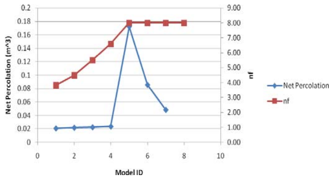
Figure 3 Influence of mesh density on solution validity
