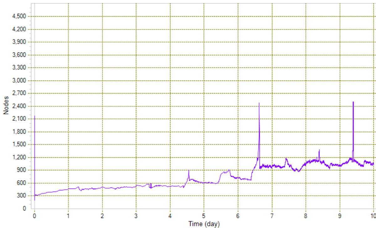
Figure 4 Number of nodes in the 1D model versus time
